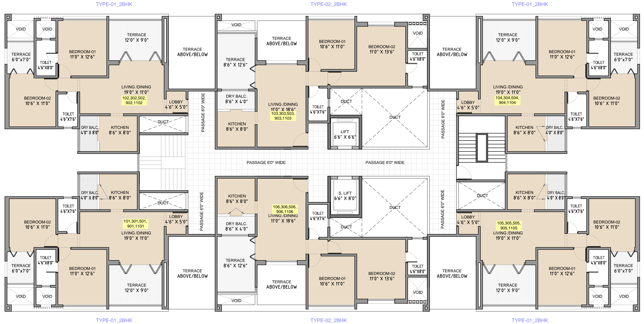
TYPICAL - ODD FLOOR PLAN 1,3,5,9,11th FLOOR PLAN BUILDING - F
